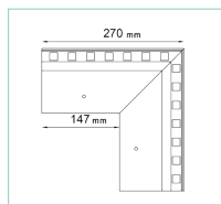
W30 90 EXTERNAL CORNER
