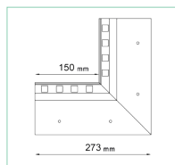
W30 90 INTERNAL CORNER
