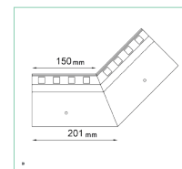
W30 135 INTERNAL CORNER
