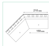
W30 135 EXTERNAL CORNER
