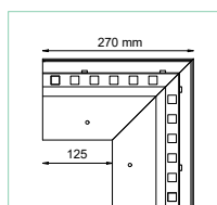
W20R 90 EXTERNAL CORNER
