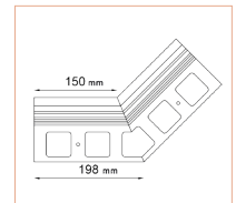
K20R 135 INTERNAL CORNER
