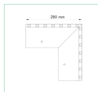
W60 90 EXTERNAL CORNER
