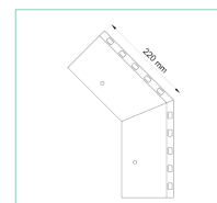
W60 135 EXTERNAL CORNER
