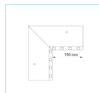
W60 90 INTERNAL CORNER
