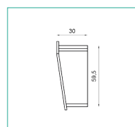
OPK301 R+L WALL PROTECTION END CAPS
