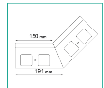
K301 135 INTERNAL CORNER
