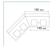
K301 135 EXTERNAL CORNER
