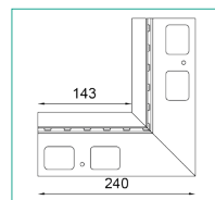
K102 90 INTERNAL CORNER
