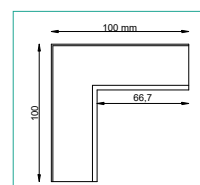
K102 RETURN PIECE
