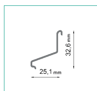
LK102 DRIP EDGE CLIP
