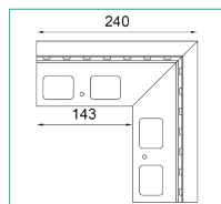
K102 90 EXTERNAL CORNER
