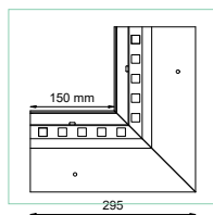
W20R 90 INTERNAL CORNER
