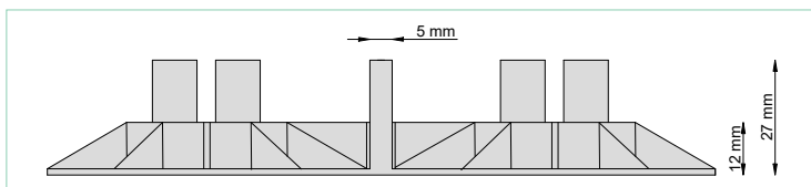
SMART pedestal with 5 mm paver spacing
