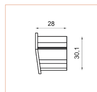
OPK20/OPK20R R+L WALL PROTECTION END CAPS
