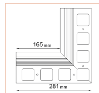
K20R 90 INTERNAL CORNER
