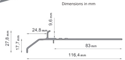
K20 SIMPLE Drip edge profile
