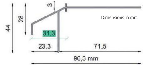
K100R ECO+ Drip edge profile
